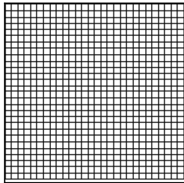
Input neurons
