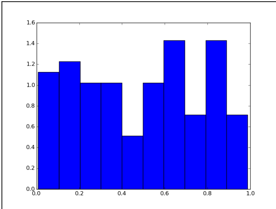
Uniform distribution
