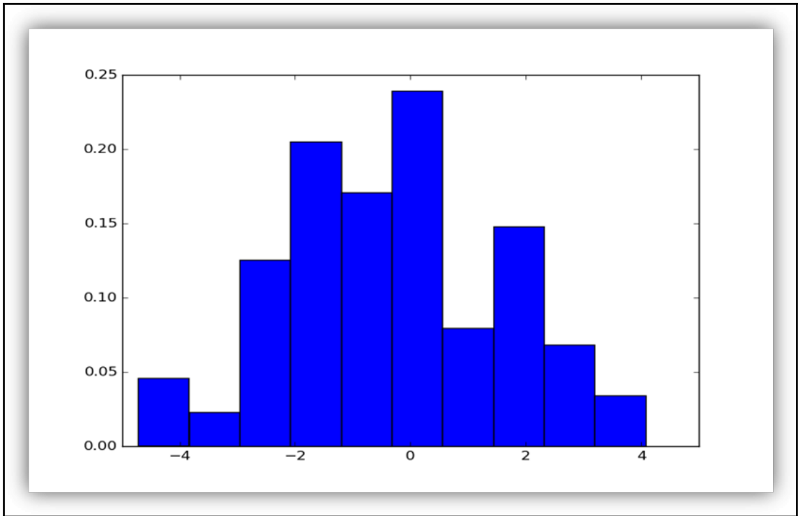
Normal distribution
